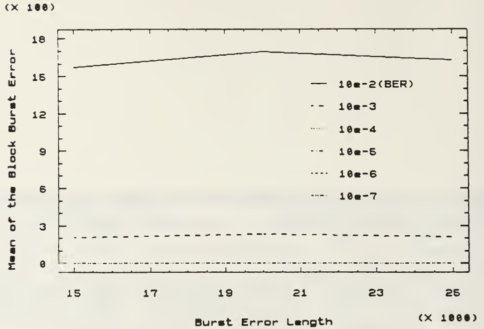
Figure B.1: Distribution of CRC-4(2048 Bits)
